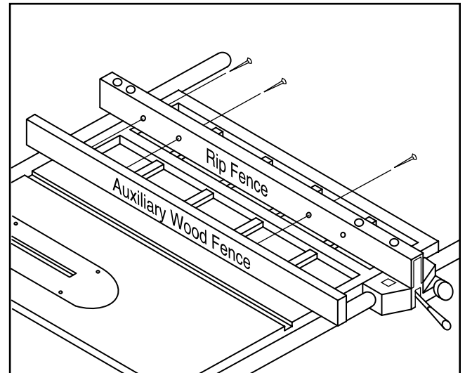
Figure 39. Attaching a sacrificial fence.
