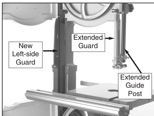
Figure 5. Extension block components.
