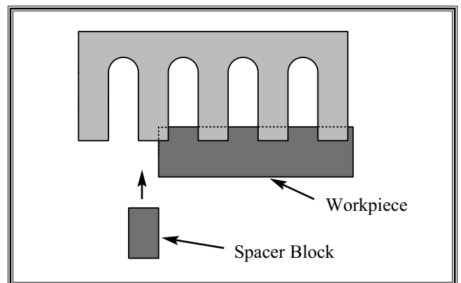
Figure 3. Spacer block.
