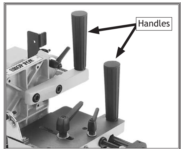
Figure 5. Handles installed.
