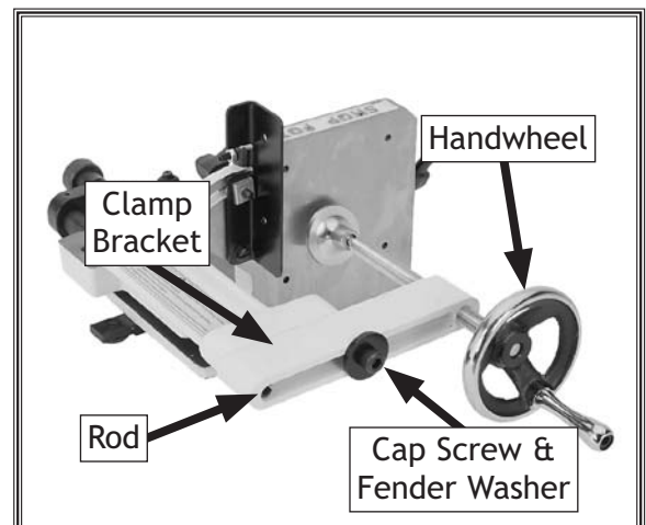
Figure 6. Clamp shoe, bracket, and handwheel installed.
