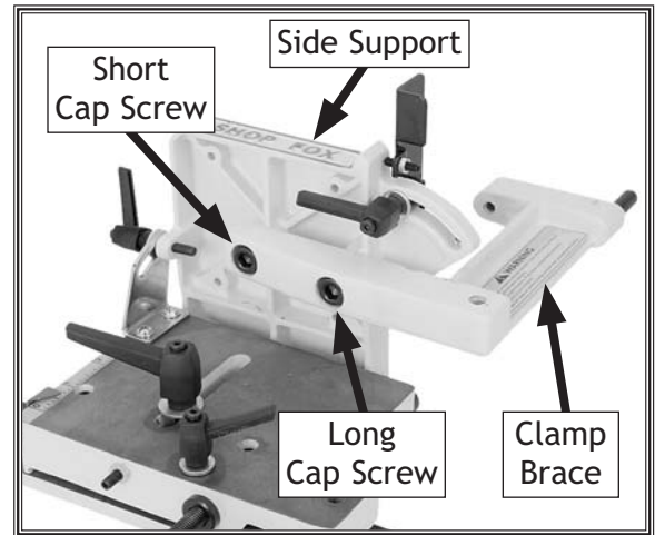
Figure 4. Clamp brace installed.
