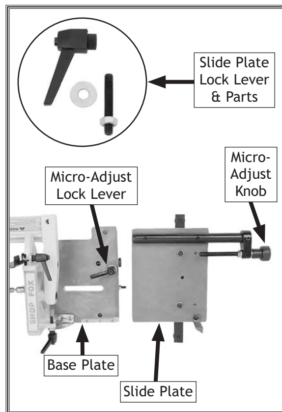
Figure 7. Slide and base plates separated.
