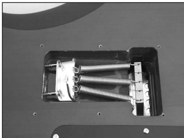
Figure 44. Spring adjustment.
