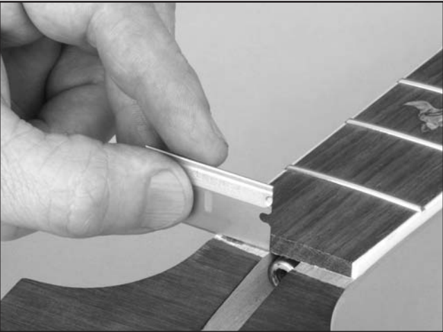
Figure 29. Cleaning out the nut slot.
