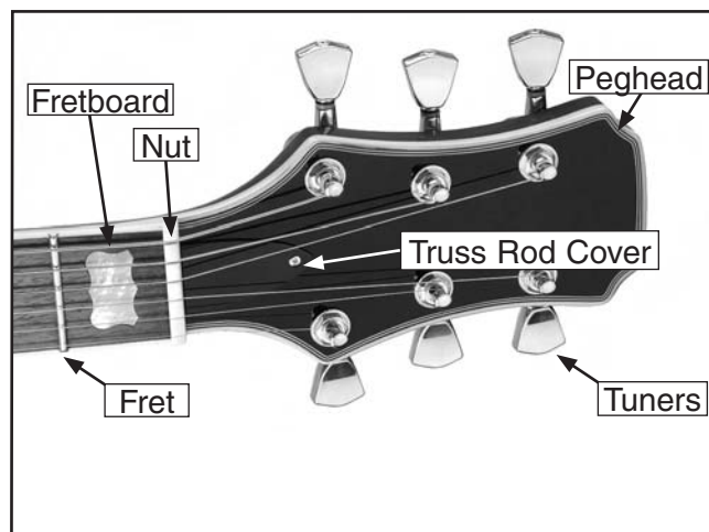
Figure 11. Peghead identification.
