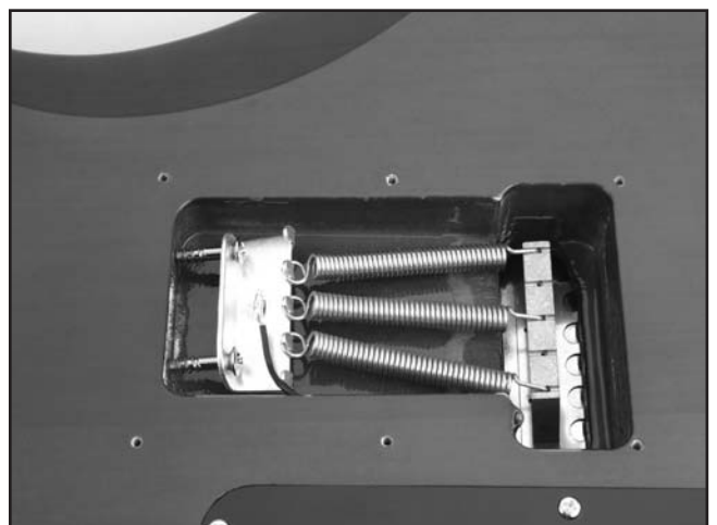
Figure 28. Correct spring placement.
