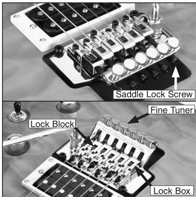
Figure 34. Bridge components.
