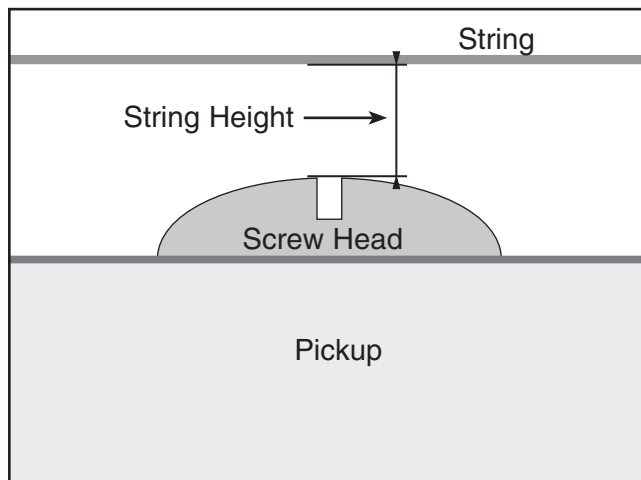
Figure 42. String heights over the pickup.
