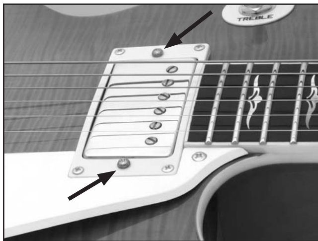
Figure 43. Pickup height adjustment.
