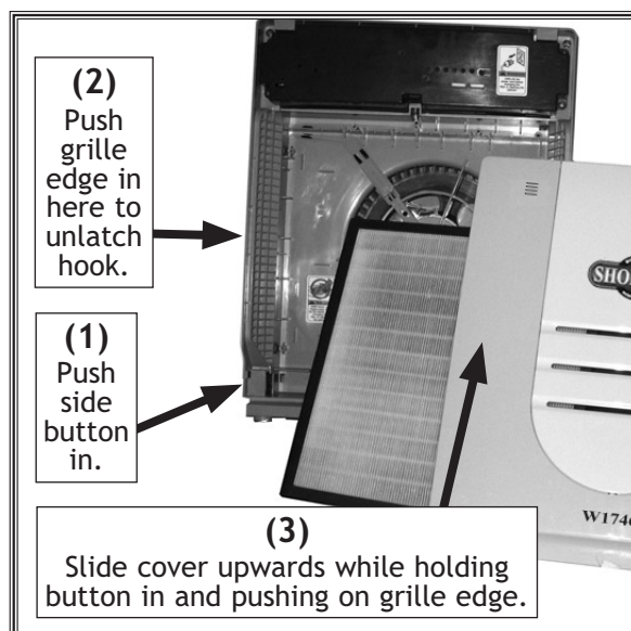
Figure 1. Filter access.
