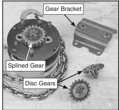
Figure 3. Gears exposed.
