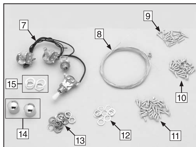
Figure 3. H6082/3 guitar parts.
