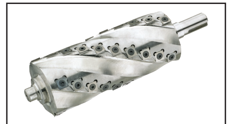
Spiral Cutterhead from G0656PX
