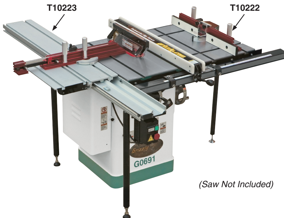
Angled Cuts with Slider
