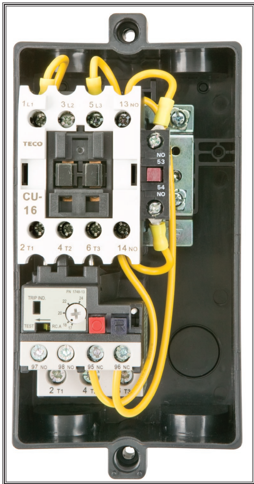
Figure 1. Model D4153 magnetic switch.
