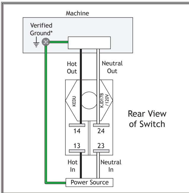
Figure 2. D4160 wiring diagram.
