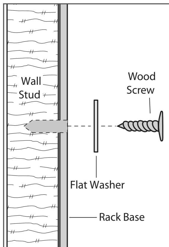
Figure 2. Wall stud installation.
