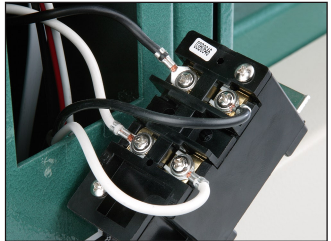
Figure 55. Power switch.
