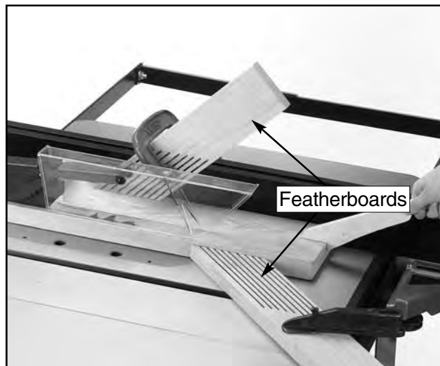
Figure 4. Featherboards.
