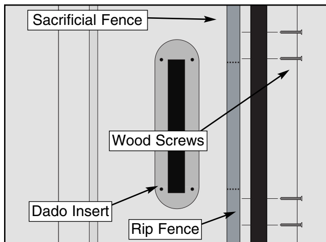
Figure 35. Sacrificial fence.
