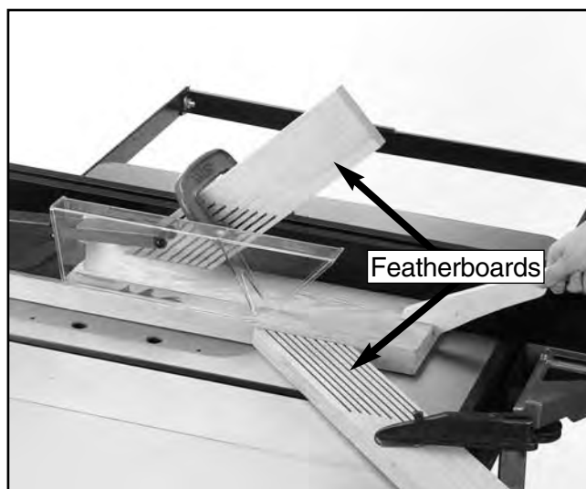
Figure 4. Featherboards.
