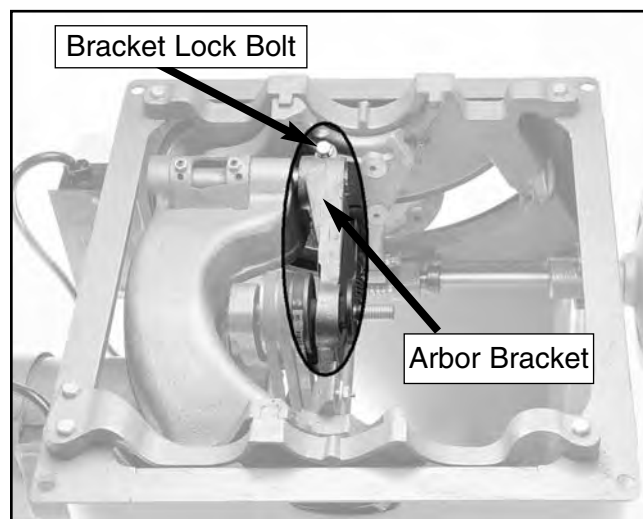
Figure 46. Adjusting arbor bracket.
