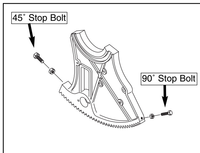
Figure 40. Geared trunnion.
