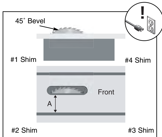
Figure 43. 45° blade parallelism measurement.
