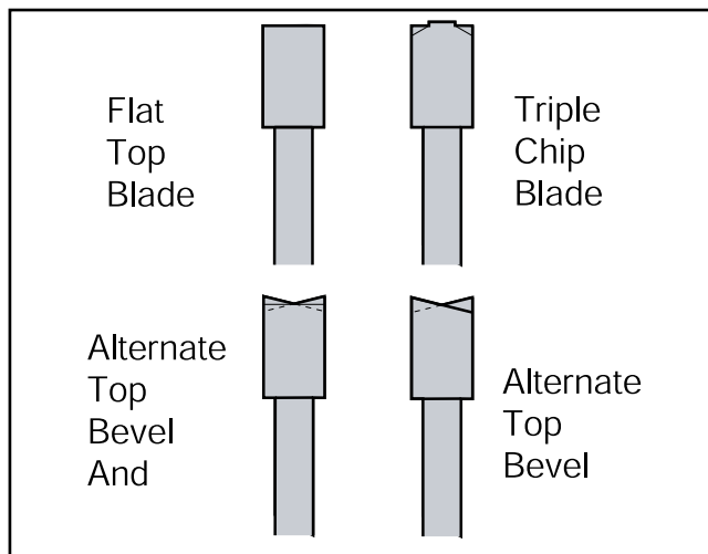
Figure 30. Various saw tooth cutting profiles.
