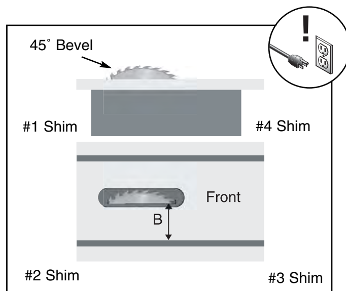
Figure 44. 45° blade parallelism measurement.
