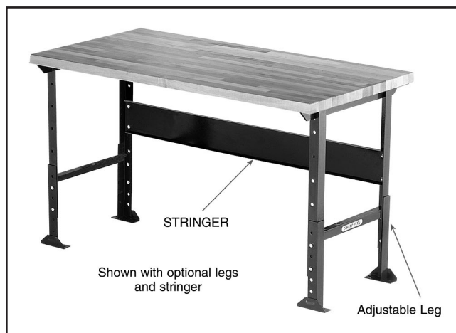
Example of Maple Workbench Top mounted on legs.
