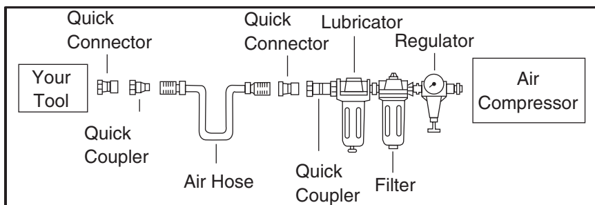
Figure 2. Typical filter/lubricator/regulator installation order.
