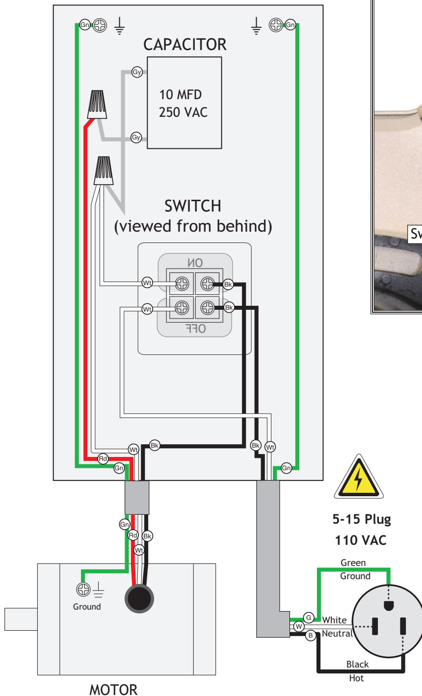
Figure 56. W1749 switch wiring.
