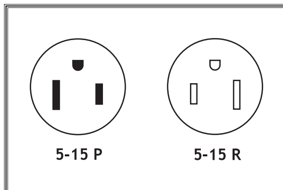
Figure 8. Typical 110V 3-prong plug and outlet.
