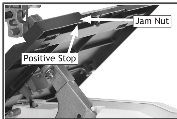
Figure 18. Positive stop.
