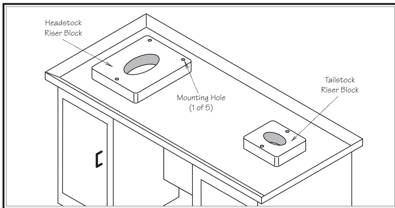
Figure 1. Orientation of riser blocks relative to lathe and stand.
