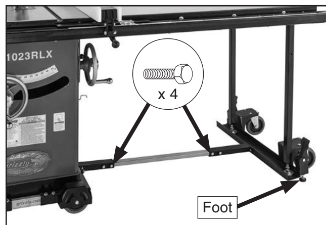
Figure 11. Extension kit attached to Model T33447 Mobile Base.
