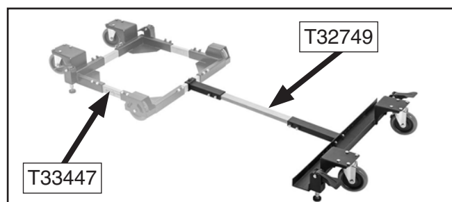
Figure 1. Assembled T32749 Extension Kit attached to T33447 Mobile Base.
