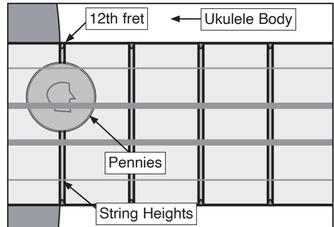
Figure 29. Correct 12th fret string heights.
