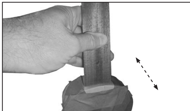
Figure 5. Sanding neck.
