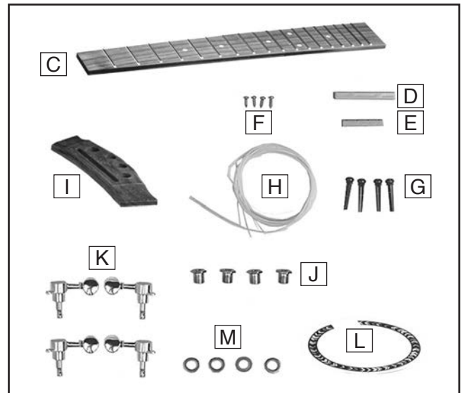
Figure 2. Ukulele components.
