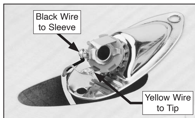
Figure 14. Wires soldered to output jack tabs.
