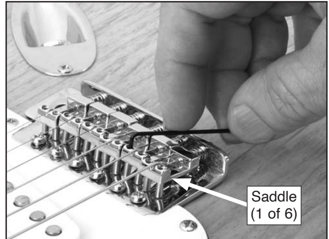
Figure 28. Example of adjusting string height.
