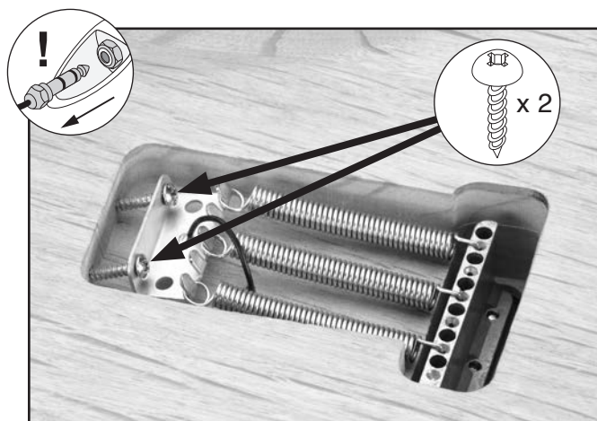
Figure 32. Location of tremelo springs.
