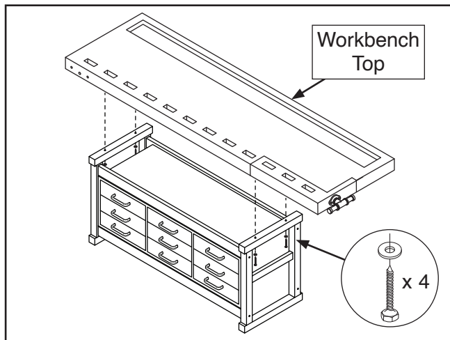
Figure 9. Attaching workbench top to frame.
