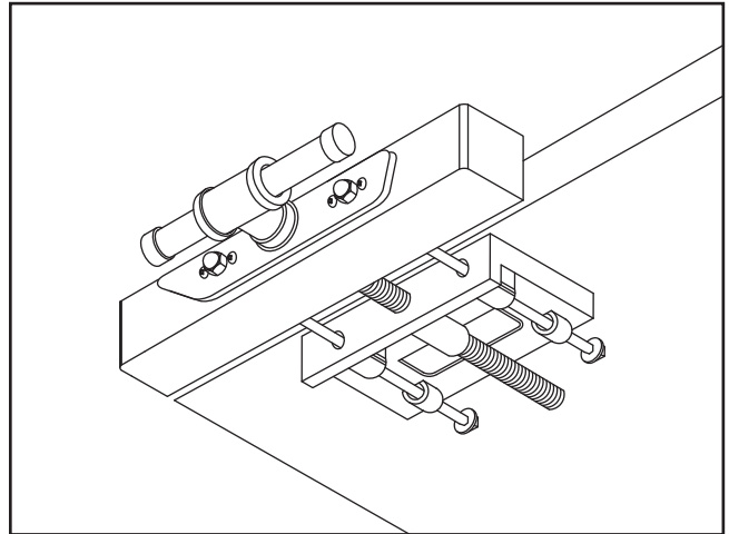
Figure 13. Vise assembly installed.
