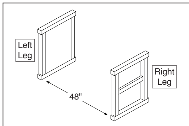
Figure 4. Positioning workbench legs.
