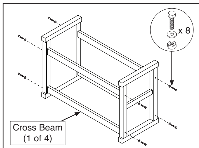
Figure 5. Attaching crossbars.
