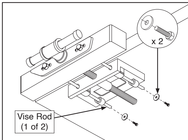
Figure 12. Installing vise assembly.
