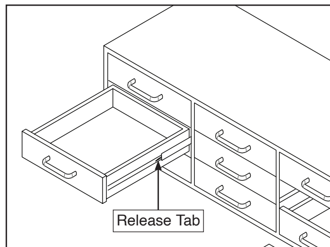
Figure 7. Removing drawers.
