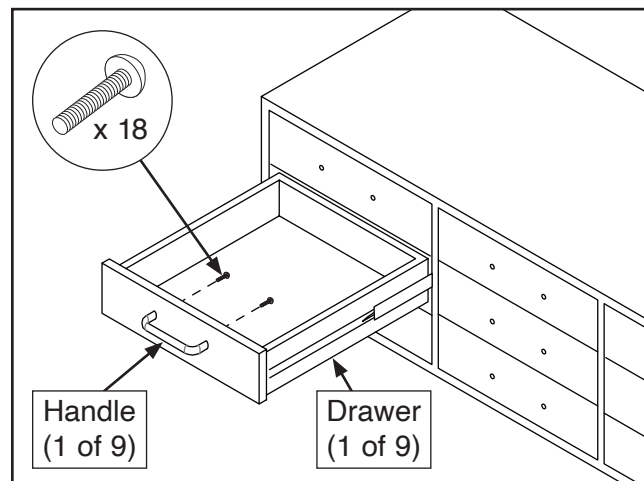
Figure 6. Installing handles.
