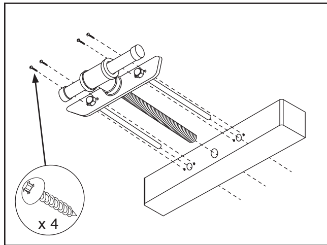
Figure 10. Assembling vise components.
