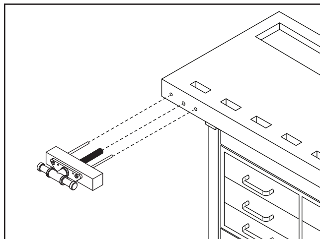
Figure 11. Inserting face vise assembly into workbench holes.
