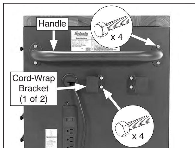
Figure 3. Handle and cord-wrap brackets installed.
