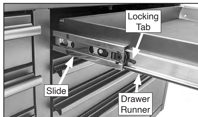
Figure 5. Location of drawer components (left side shown).
