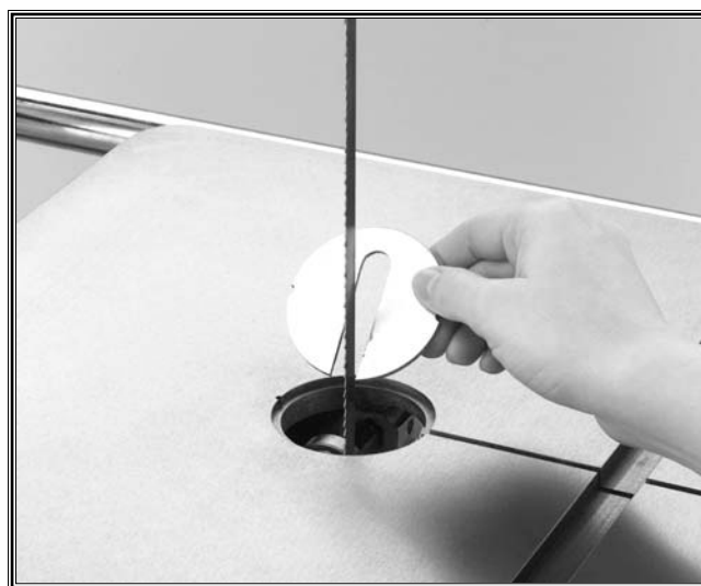
Figure 29. Removing table insert.
