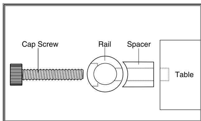
Figure 21. Rail assembly.
