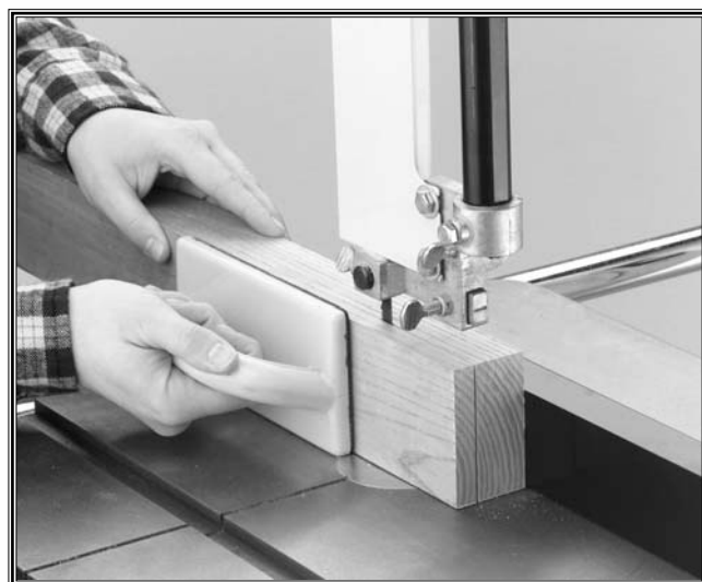
Figure 53. Resawing.
