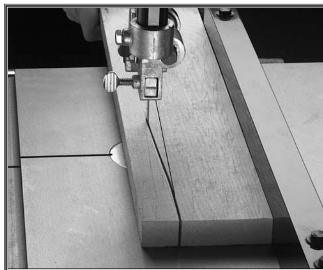
Figure 47. This rip cut illustrates excessive blade lead.
