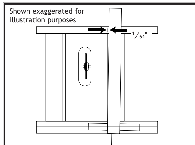
Figure 10. Lead adjustment.
