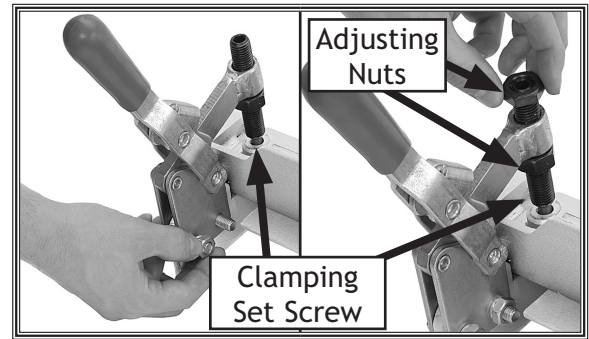
Figure 4. Clamp installation.
